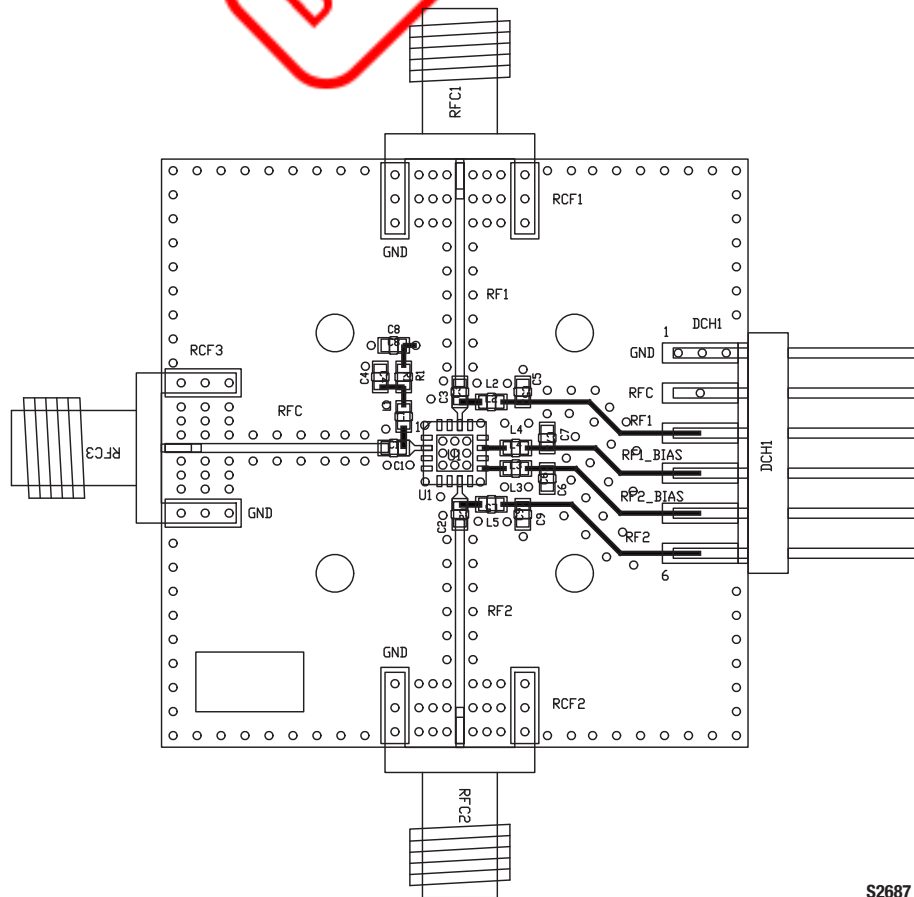
Figure 14. SKY12211-478LF Evaluation Board Assembly Diagram
