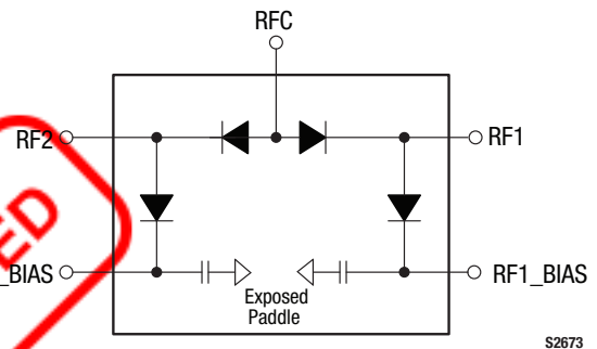
Figure 1. SKY12211-478LF Block Diagram
