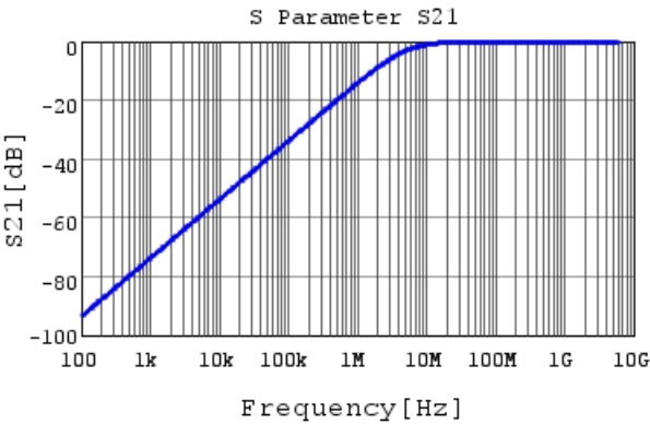
GRM033R71C331KA01 S21 DC0V,25degC
