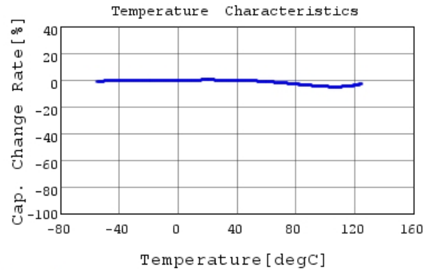
GRM033R71C331KA01 C-Temp. capchange, DC0.0V,
