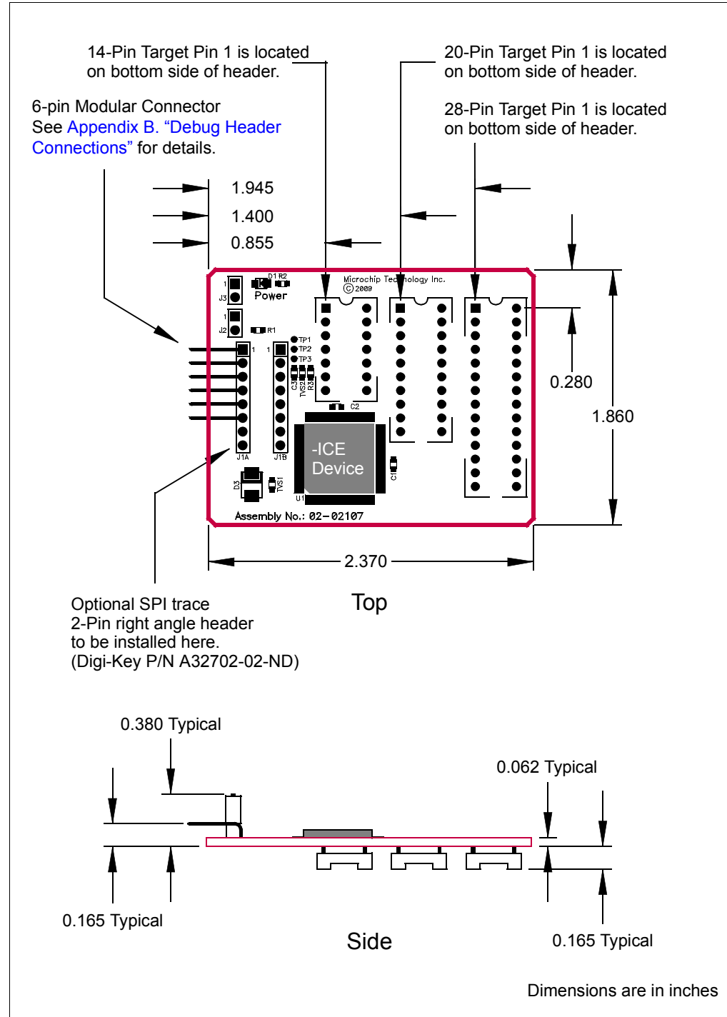
FIGURE 2-11: DIMENSIONS - AC244028
