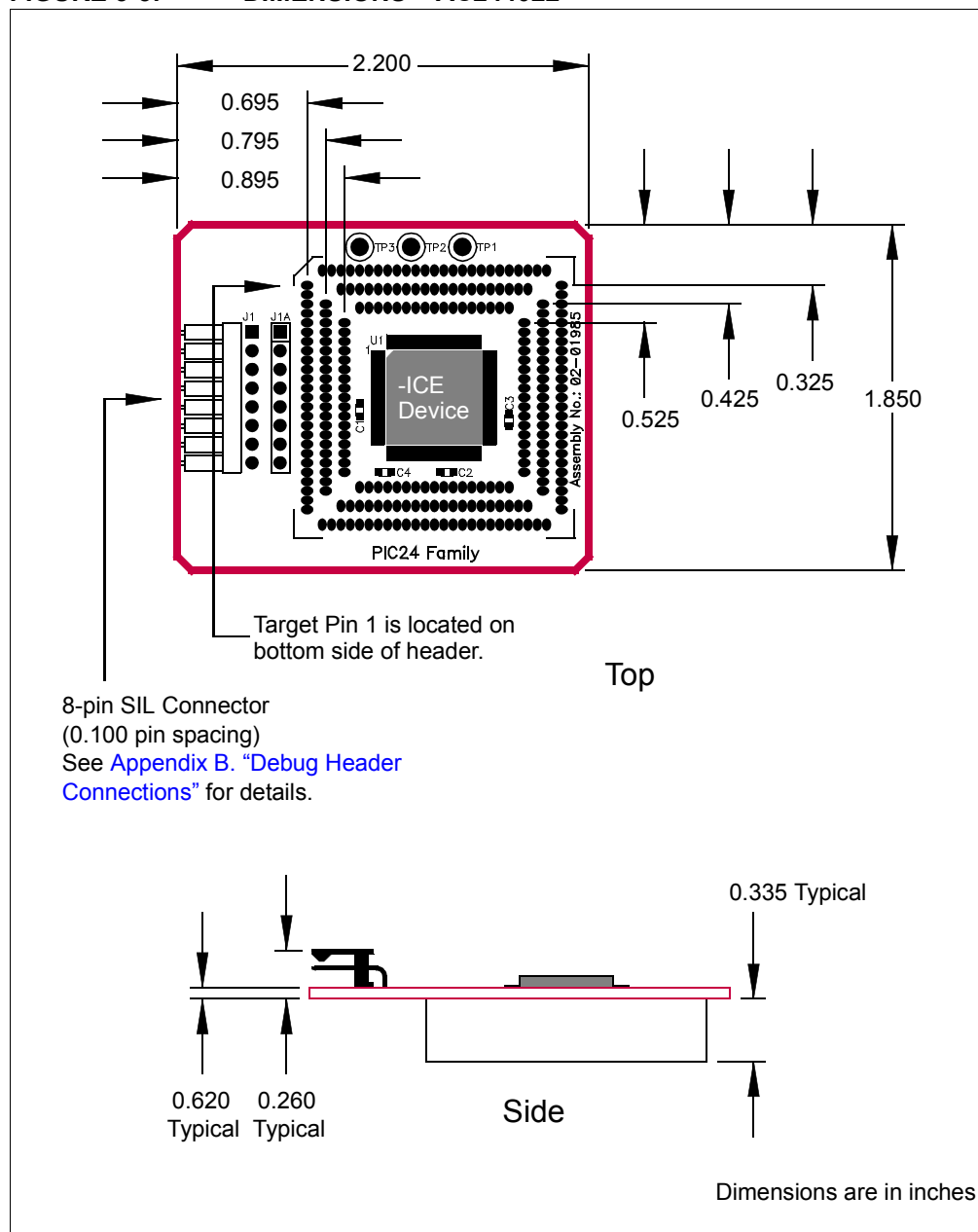
FIGURE 3-5: DIMENSIONS – AC244022
