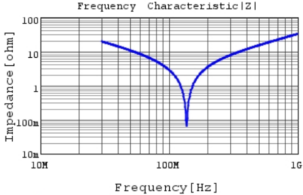
RCE5C2J271J1K1H03B |Z| DCOV, 25degC
