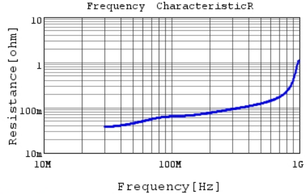
RCE5C2J271J1K1H03B R DCOV, 25degC
