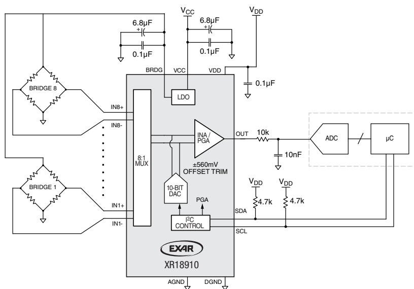
Figure 1. Typical Application
