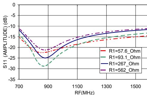
S11 (AMPLITUDE,dB) Vs. Frequency and R1 Values
