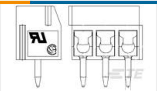
TE Part #1776275-2 2P TB ,90deg,VT,3.5mm,Blue,w /interlock
