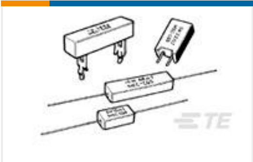
TE Part #2-1623779-8 SQB20 1K0 5% (WIRE)
