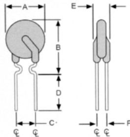
RS90-010 ~ RS90-090 Lead Size: 24AWG, 0.51 mm Diameter
