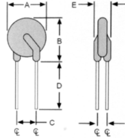
RS90-110 ~ RS90-375 Lead Size: 20AWG, 0.81 mm Diameter
