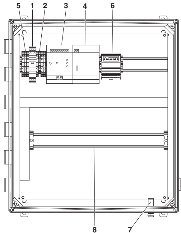
Figure 4 RTU READY EX UPS 181610 components
