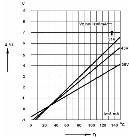
Fig 14. Change of Zener Voltage vs T_j
