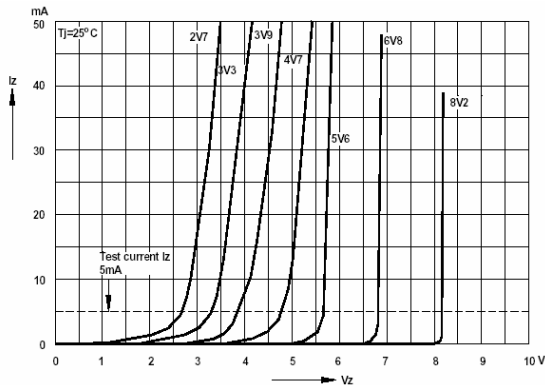
Fig 1. Breakdown Characteristics @ T_j = \text{Constant} (pulsed)
