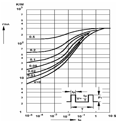
Fig 5. Pulse Thermal Resistance vs Pulse Duration
