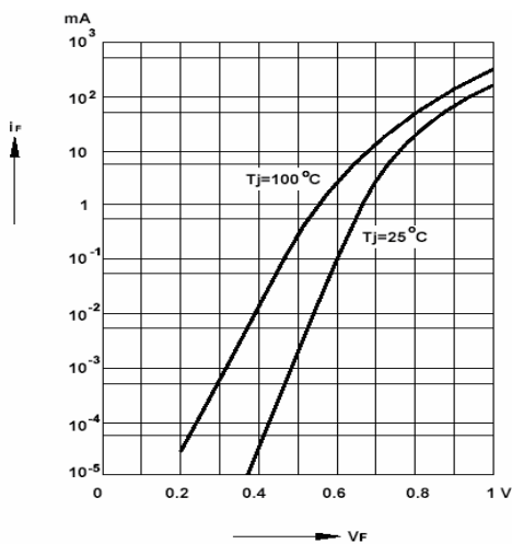
Fig 3. Forward Characteristics
