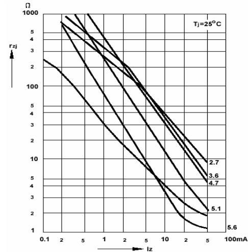
Fig 6. Dynamic Resistance vs Zener Current
