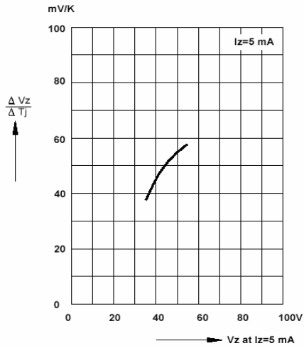
Fig 13. Temperature Dependence of Zener Voltage vs Zener Voltage
