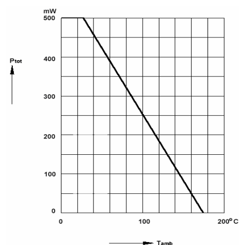
Fig 4. Admissible Power Dissipation vs T_A
