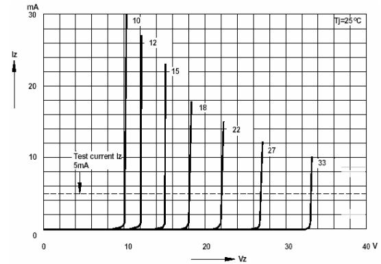
Fig 2. Breakdown Characteristics @ T_j = \text{Constant} (pulsed)
