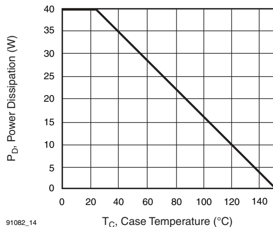
Fig. 14 - Power vs. Temperature Derating Curve
