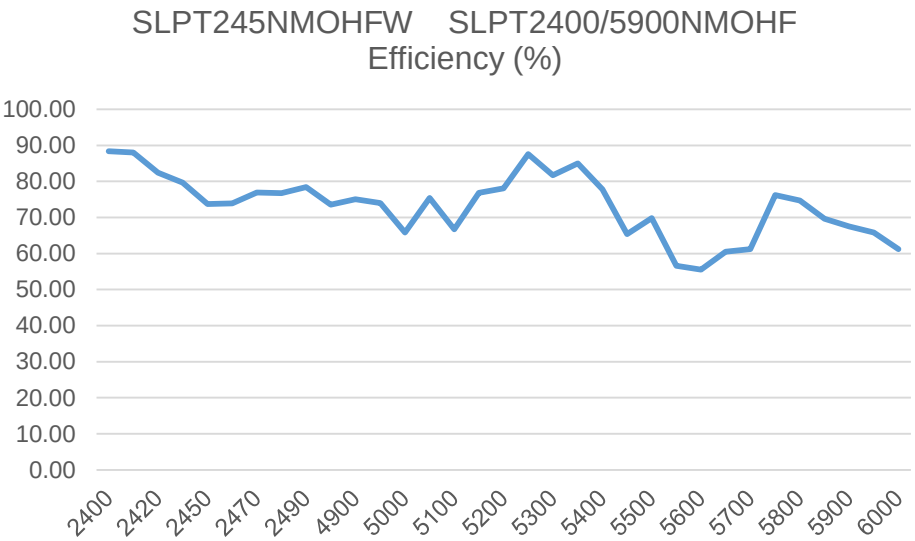
Efficiency(%)
