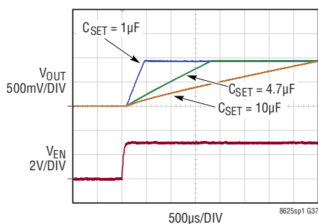
Soft-Start Waveforms
