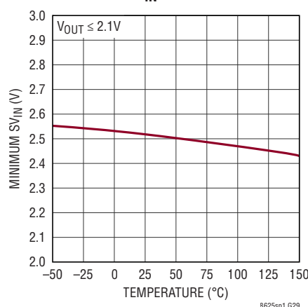
Minimum SV_{IN}
