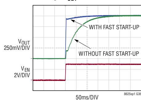
Start-Up Time with and without Fast Start-Up Circuitry for Large C_{\text{SET}}
