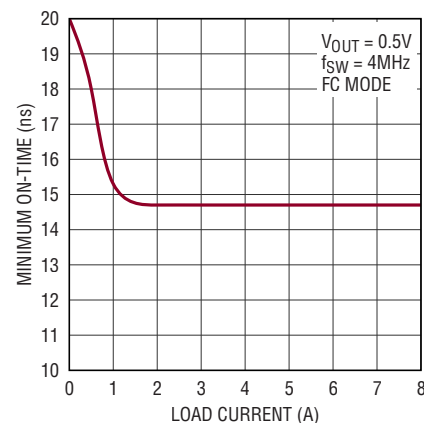
Minimum On-Time vs Load
