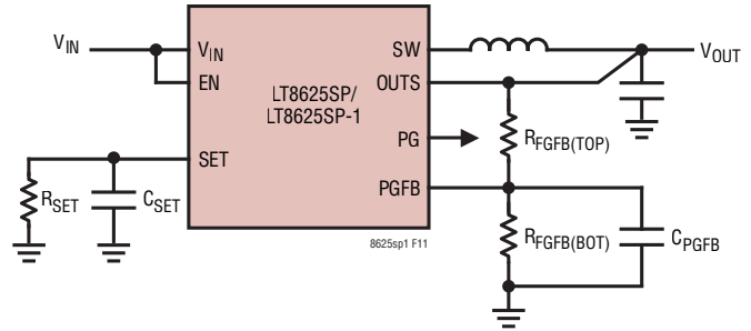
Figure 11. Schematic with C_{\text{PGFB}}
