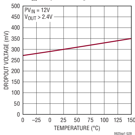
SV_{IN} Dropout Voltage
