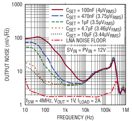
Noise Spectral Density vs C_{\text{SET}}
