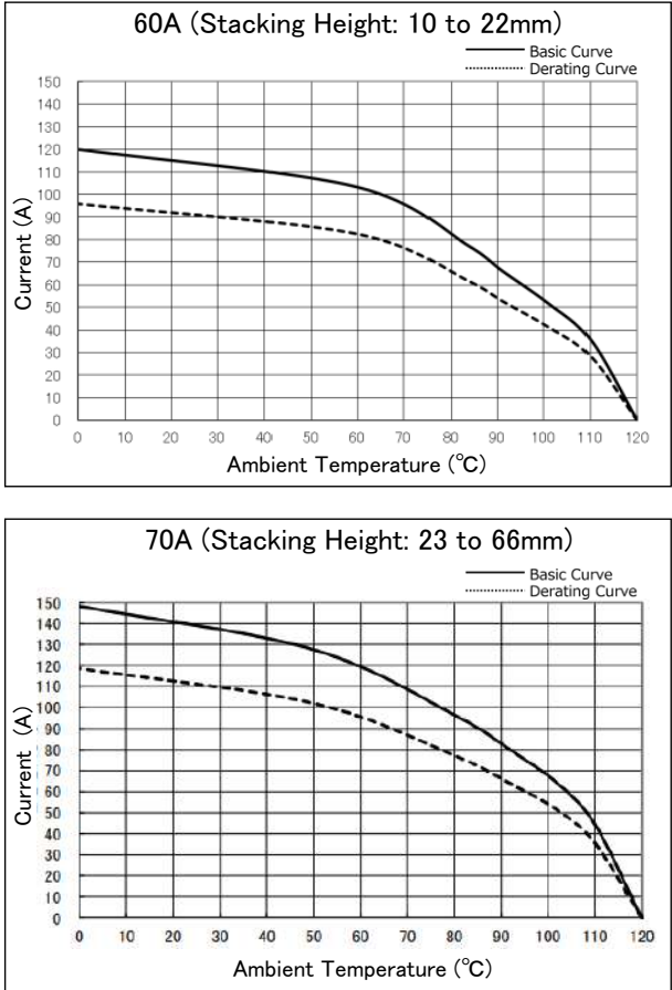
Electric Capacity Test (Derating Curve)
