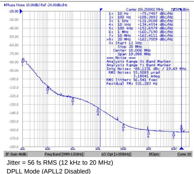
Figure 8. 156.25-MHz Output Phase Noise (APLL1)
