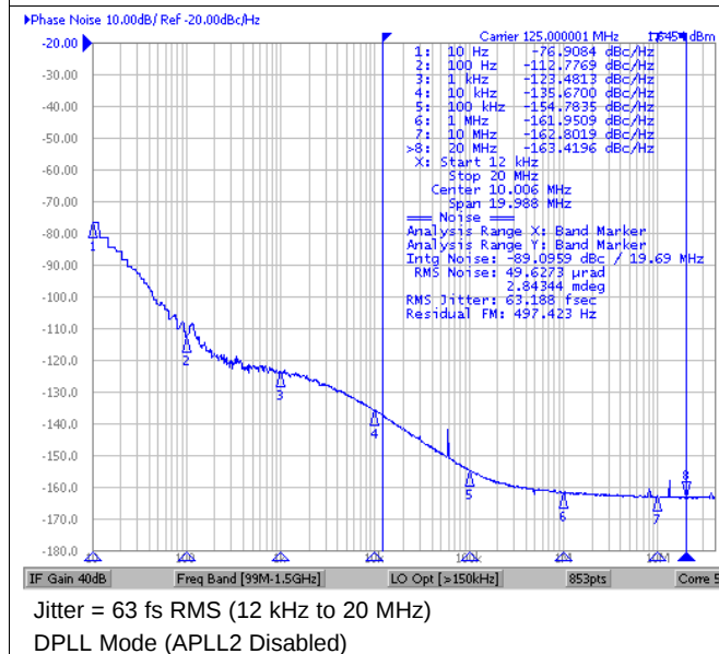
Figure 9. 125-MHz Output Phase Noise (APLL1)
