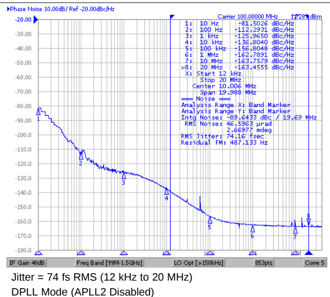
Figure 10. 100-MHz Output Phase Noise (APLL1)
