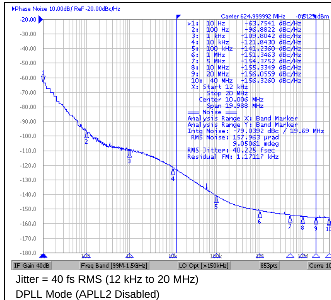
Figure 7. 625-MHz Output Phase Noise (APLL1)
