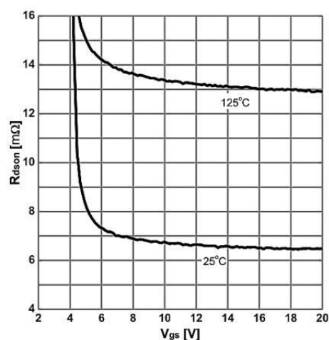
Figure 10. On-state resistance vs. Vgs characteristics
