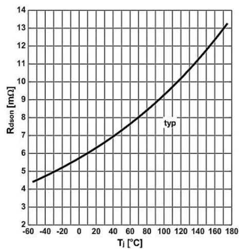
Figure 8. On-state resistance vs. Junction temperature
