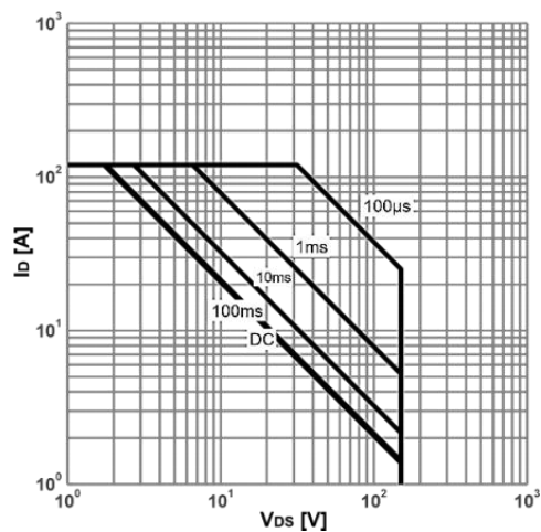
Figure 1. Power dissipation
