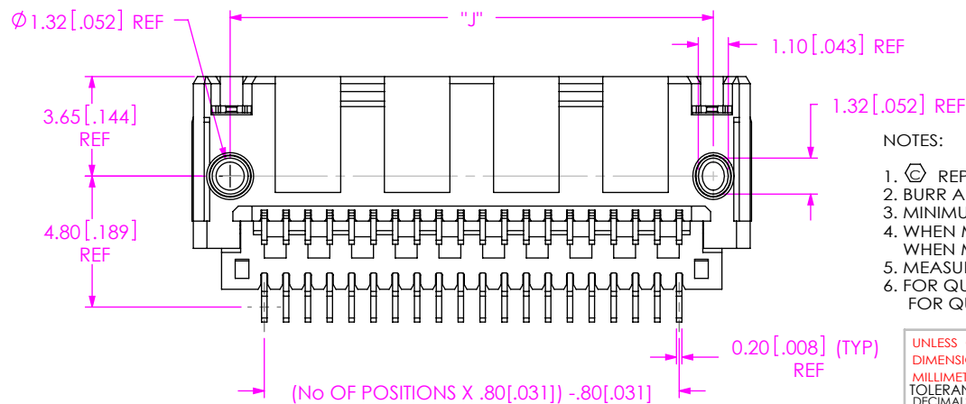
FIG 1 (LSEM-120-XX-DH-A-S-XX SHOWN)
