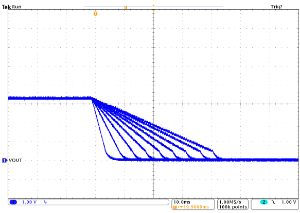
Figure 10: Simultaneous Shut-Down
