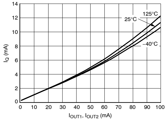
Figure 14. I_Q versus I_{OUT} ( V_{OUT1} & V_{OUT2} )
