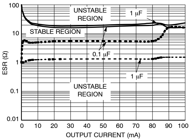
Figure 30. V_{OUT2} ( 2.5\ \text{V} ) Output Capacitor ESR ( 0.1\ \mu\text{F} / 1\ \mu\text{F} )
