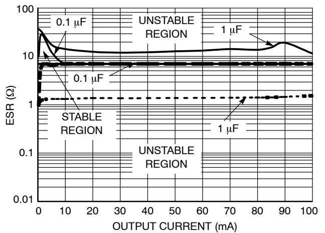
Figure 31. V_{OUT2} ( 1.8\ \text{V} ) Output Capacitor ESR ( 0.1\ \mu\text{F} / 1\ \mu\text{F} )
