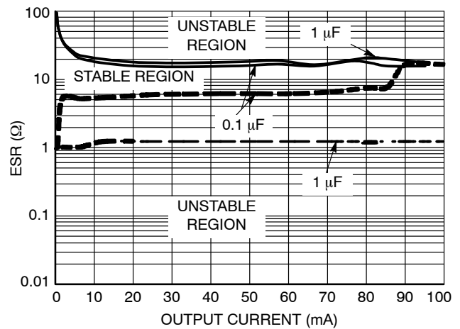
Figure 29. V_{OUT2} ( 2.6\ \text{V} ) Output Capacitor ESR ( 0.1\ \mu\text{F} / 1\ \mu\text{F} )
