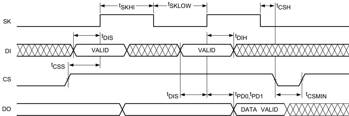
Figure 3. Synchronous Data Timing
