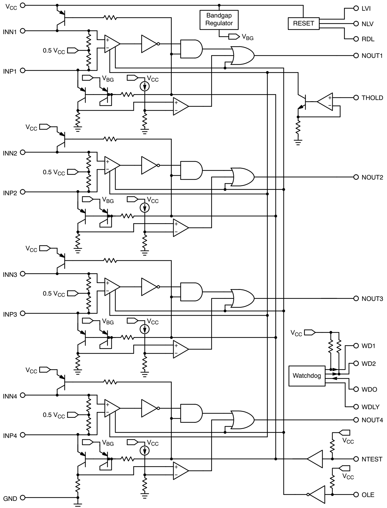
Figure 2. Block Diagram
