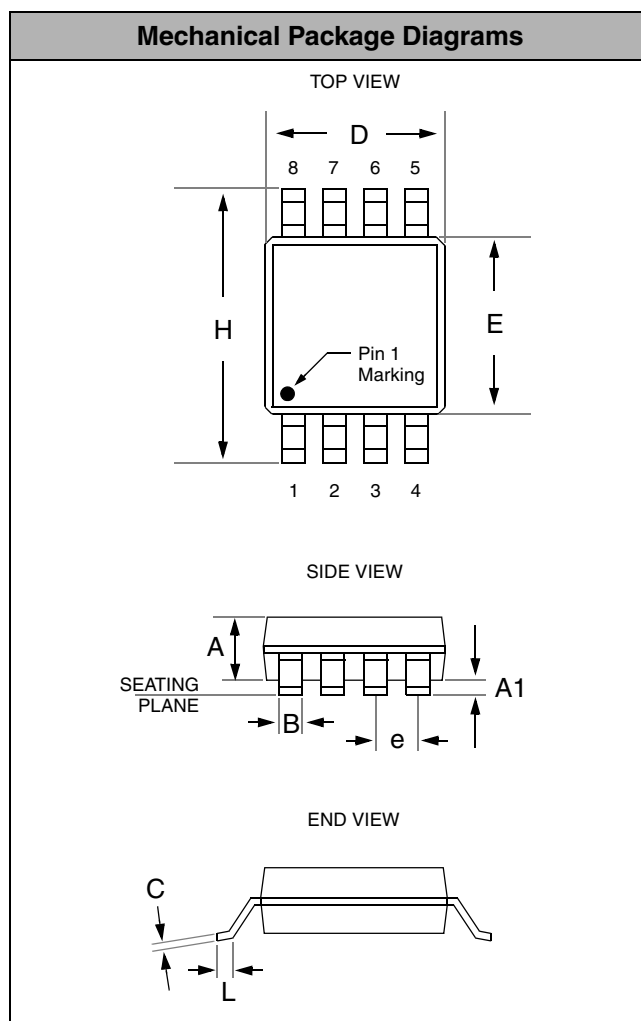
Dimensions for MSOP-8 Package
