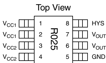
8-pin MSOP CMPWR025R
