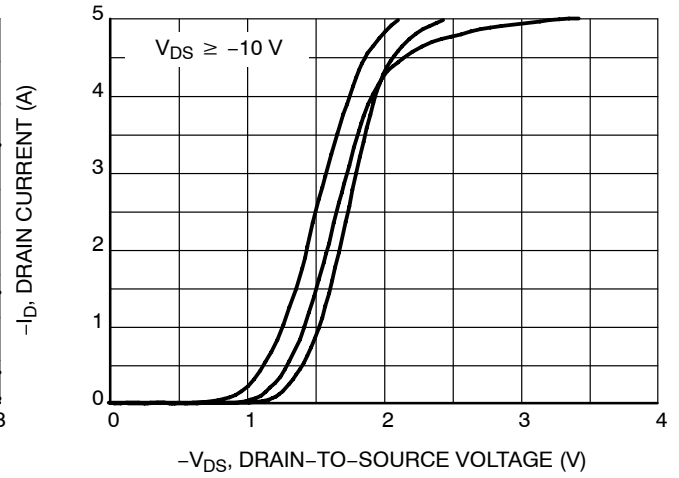
Figure 2. On-Region Characteristics
