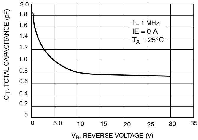
Figure 4. Total Capacitance
