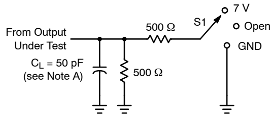
LOAD CIRCUIT
