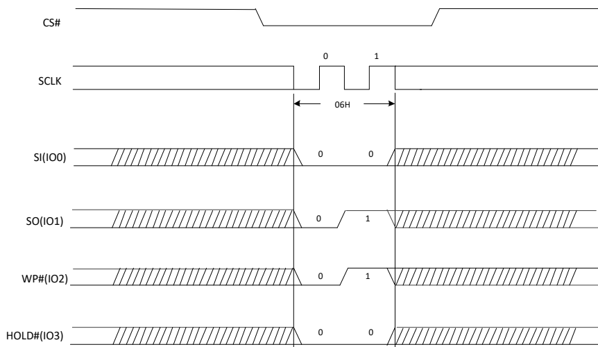
Figure 2a. Write Enable Sequence Diagram (QPI)
