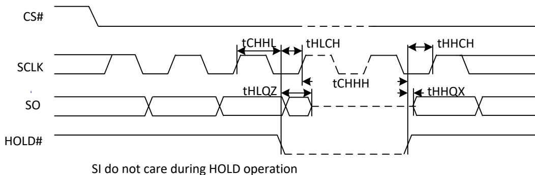
Figure 41. Hold Timing
