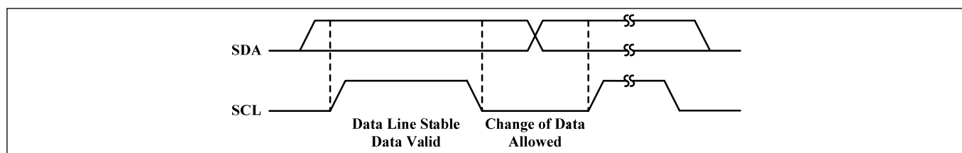
Figure 13 Bit Transfer
