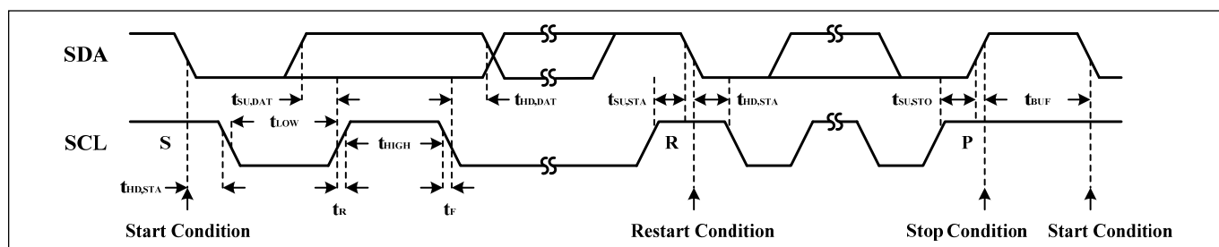
Figure 12 Interface Timing
