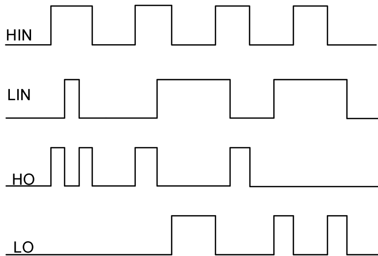
Figure 5. NSG2304 Input and output timing waveform
