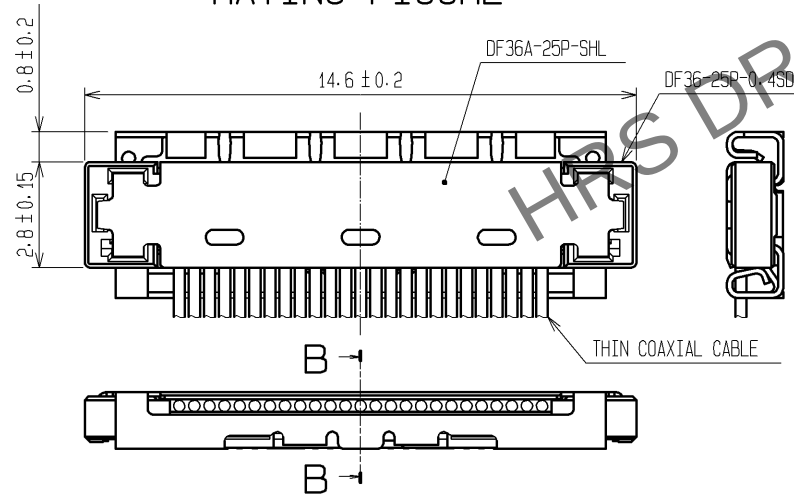
MATING FIGURE
