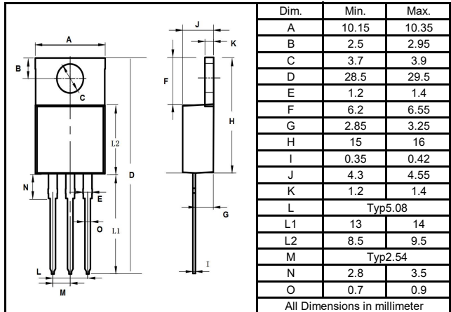
TO-220AB
