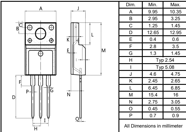
TO-220F
