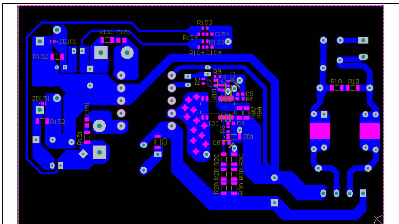
Figure 5 Bottom side copper and component legend
