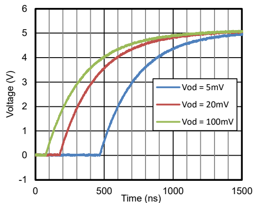
Figure 3. Propagation Delay, Low to High
