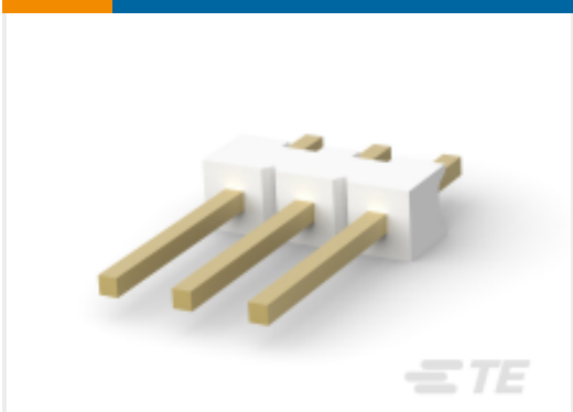
TE Part #3-644456-7 Polyester Vertical PCB Header: 2.54 mm, Breakaway, MTA 100
