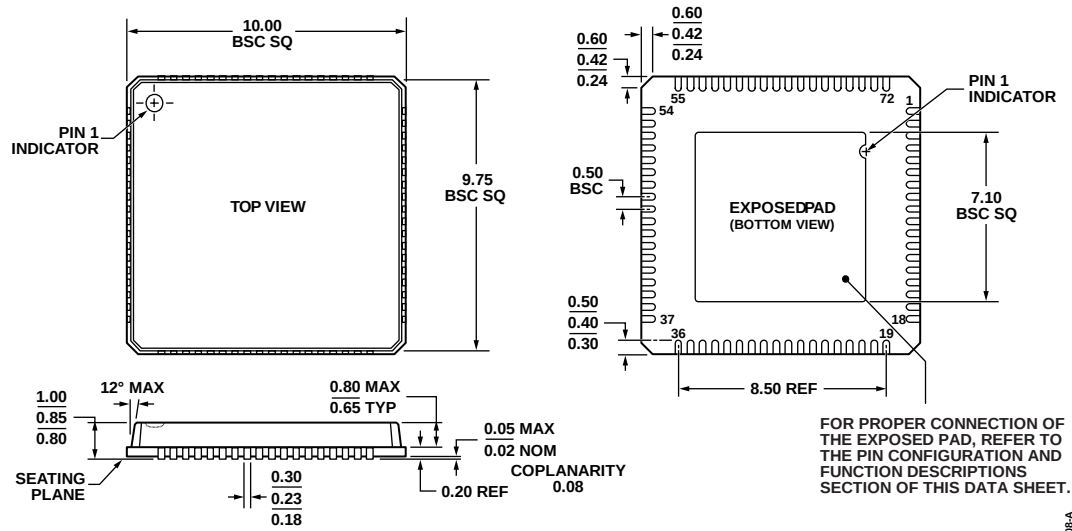
Figure 104. 72-Lead Lead Frame Chip Scale Package [LFCSP_VQ] 10 mm x 10 mm Body, Very Thin Quad (CP-72-4) Dimensions shown in millimeters
