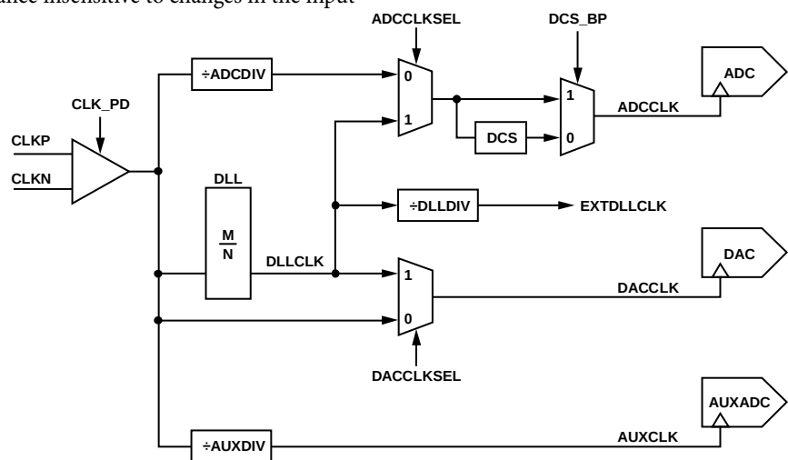
Figure 65. Clock Distribution Diagram
