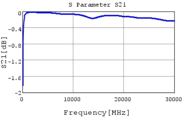
GRM0115C1E220GE01 S21 DCOV, 25degC
