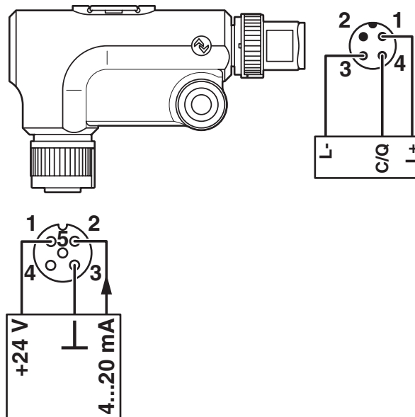
Connection diagram
