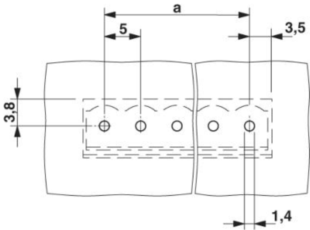
Drilling diagram
