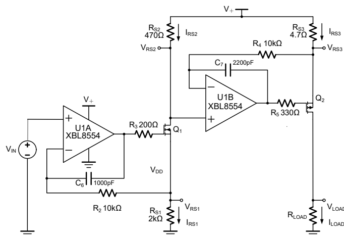
Figure 8. Bidirectional Current-Sensing
