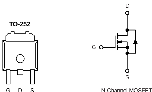
N-Channel MOSFET
