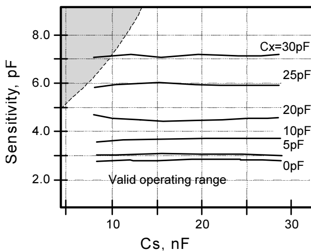
Figure 4-3 Low Gain Sensitivity and Range @ Vdd = 3V
