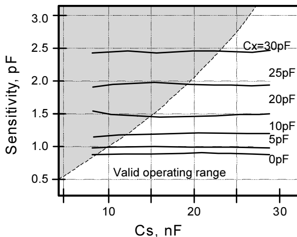
Figure 4-1 High Gain Sensitivity and Range @ Vdd = 3V
