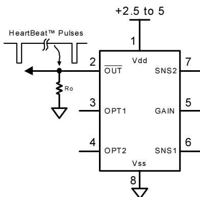
Figure 2-4 Getting HB pulses with a pull-down resistor
