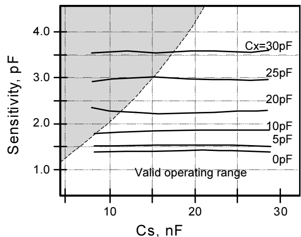
Figure 4-2 Medium Gain Sensitivity and Range @ Vdd = 3V
