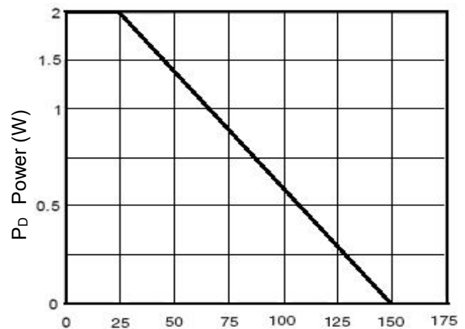
T_J -Junction Temperature( ^{\circ}C ) Figure 9 Power Dissipation
