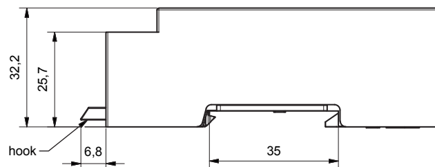
Assembly
