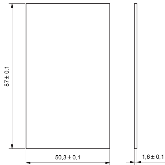
Dimension of PCB
