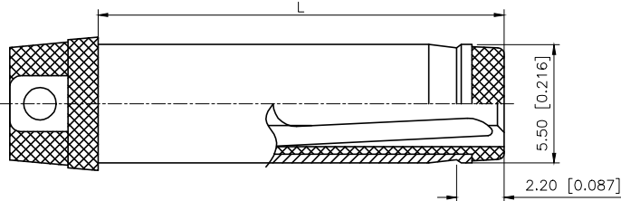
RECOMMENDED PLUG
