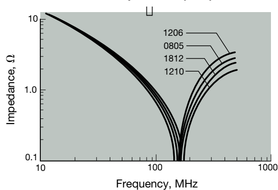
Variation of Impedance with Chip Size
