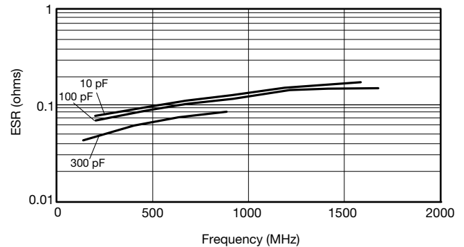
TYPICAL ESR vs. FREQUENCY
