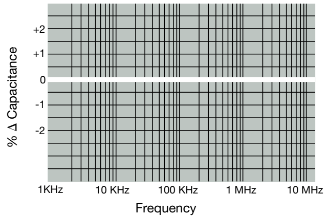
\Delta Capacitance vs. Frequency
