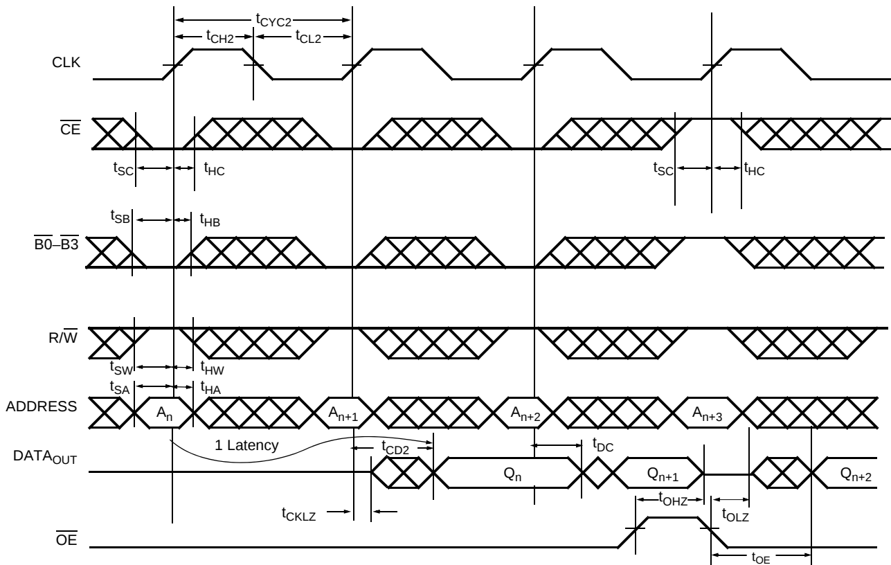
Figure 9. Read Cycle [32, 33, 34, 35, 36]
