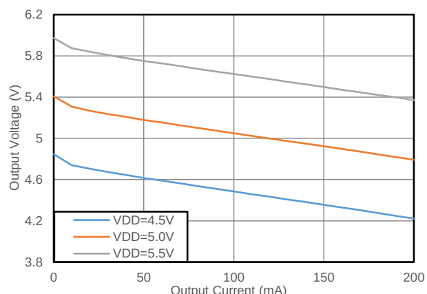
图 8.2 输出电压 vs 输出电流 (常温) (CMP6503S+CMT6870N, 5.0V to 5.0V, SEL=VDD)
