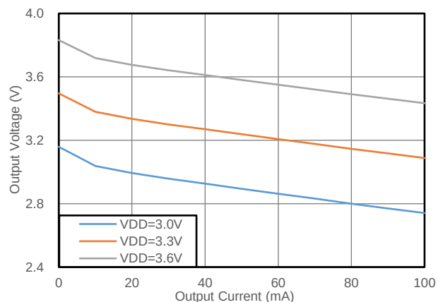
图 8.6 输出电压 vs 输出电流 (常温) (CMP6503S+CMT6870N, 3.3V to 3.3V, SEL=GND)
