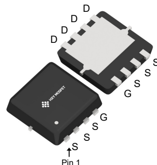
DFN3X3-8L (PQFN-8(3.1x3.1))
