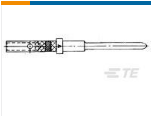
TE Part #204938-3 ARINC,PIN CONTACT,SZ 20
